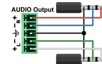
Phoenix - 2 x 6.3 (1/4") TRS
