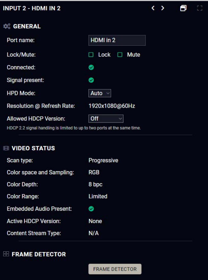
Port properties window of the HDMI video input
