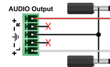
Phoenix - 2 x 6.3 (1/4") TS
