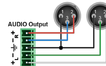
Phoenix - 2 x XLR
