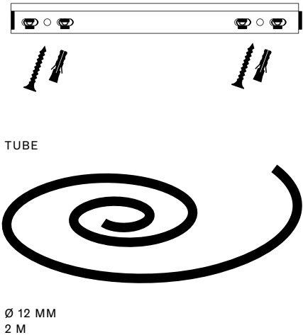
STEP 7 FIX MOUNTING RAIL
